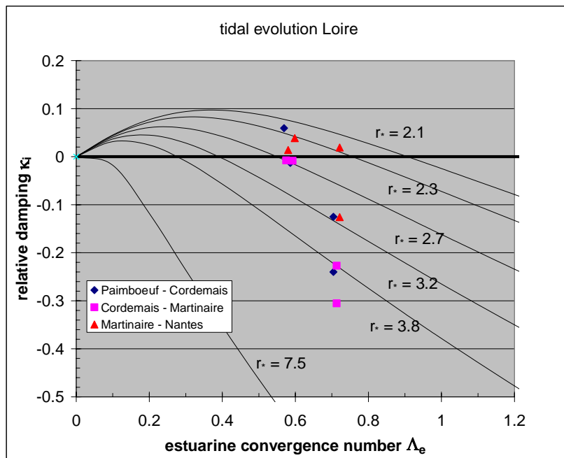
Fig. 4.19b: Tidal amplification as function of convergence number
