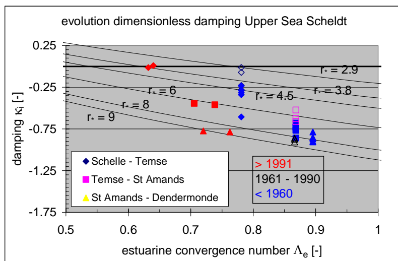
Fig. 4.53: Fits of linear solution trough observations tuning the roughness parameter r^* in the \kappa_i – \Lambda_e diagram.
