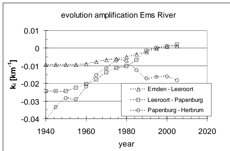
Fig. 4.5: Evolution of imaginary wave number in Ems River; note that in the remainder the data for the trajectory Papenburg – Herbrum have been ignored because of their irregularity.
