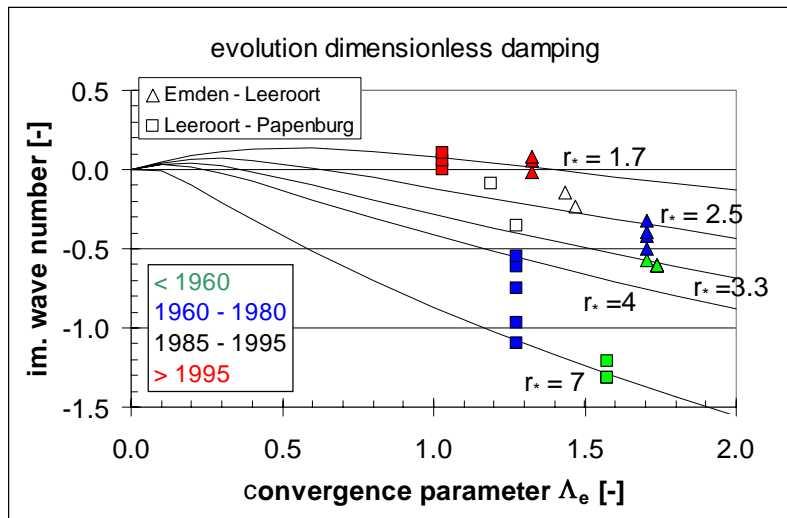
Fig. 4.7: Fits of linear solution to observed data through tuning of roughness parameter in \kappa_i - \Lambda_e diagram.
