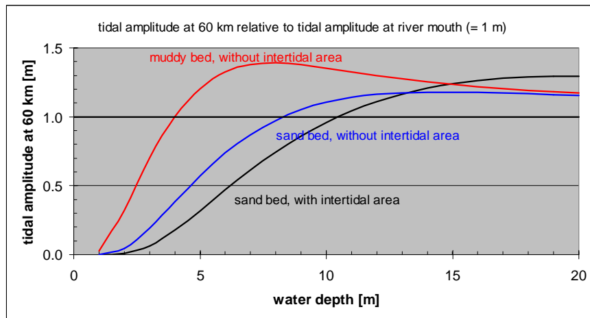
Fig. 5.2: Response of tidal amplitude as function of the presence of an intertidal area and mud in the water column, or on the River bed.
