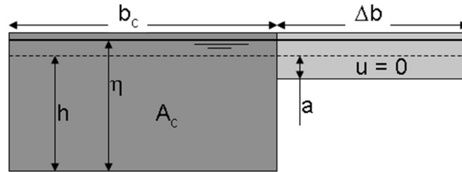
Fig. 2.1: Compound channel and definitions.
