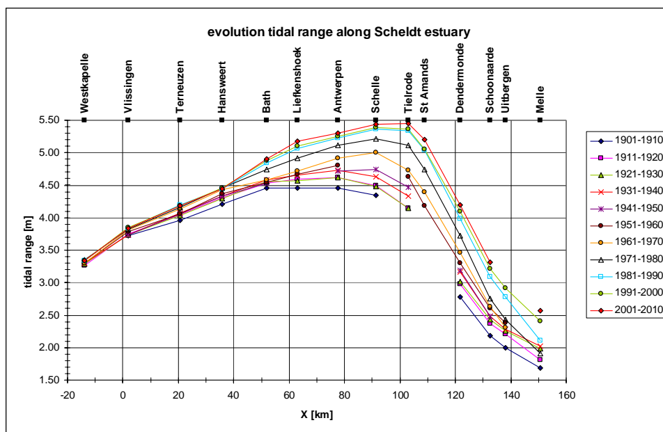
Fig. 4.41a: Evolution of tidal range along Scheldt estuary corrected for 18.6 year cycle.
