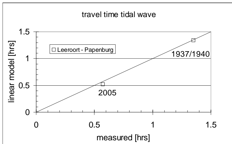
Fig. 4.10: Measured and computed travel time tidal wave along Ems River in 1940 and 2005.
