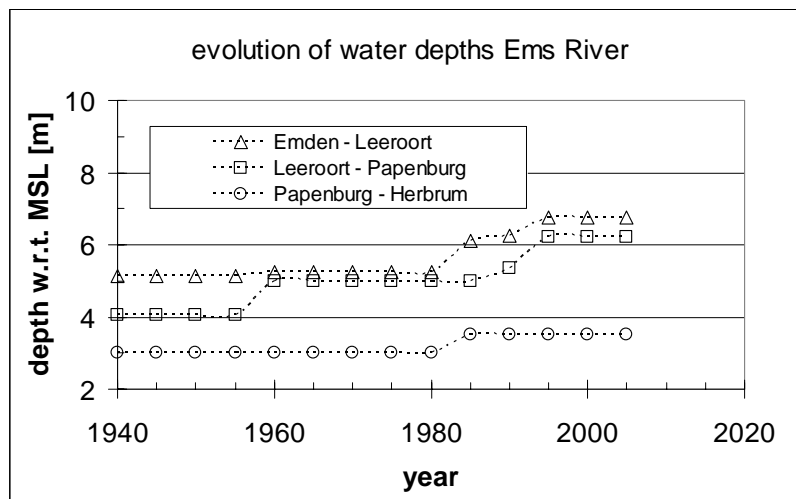
Fig. 4.3: Evolution of mean water depths in Ems River for three trajectories (water depth with respect to mean sea level at Emden).
