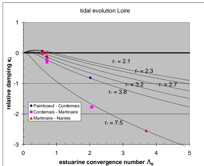
Fig. 4.19a: Tidal amplification as function of convergence number
