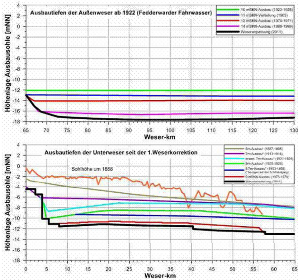
Fig. 4.37: Evolution of water depth along Weser River.
