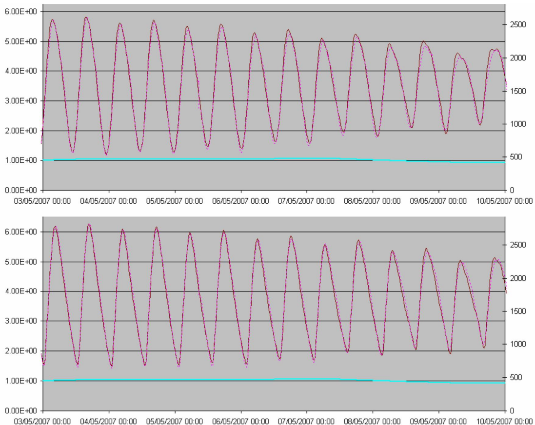
Fig. 4.21: Computed (Sogreah, 2006) tidal amplitude (vertical axis) at Donges (upper panel, km 11) and Chantenay (lower panel, km 51) showing development of steepening of the rising tide.
