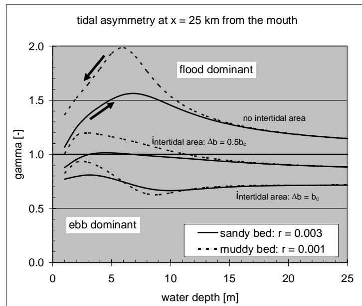
Fig. 2.13: Tidal asymmetry in converging tidal river as function of water depth and intertidal area ( \ell = \infty, L_b = 33 \text{ km} ).
