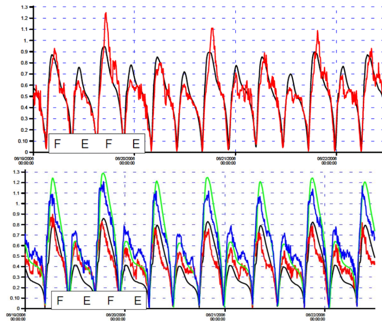
Fig. 4.35: Measured tidal asymmetry along Elbe River; upper panel: near Brunstüttel; lower panel: near Schulau (after BAW, 2011)
