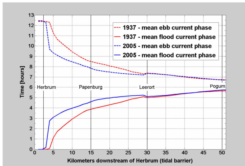
Fig. 4.9: Measured travel time tidal wave along Ems River (Herrling, 2007).
