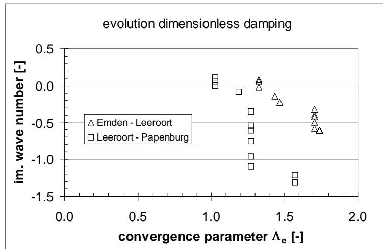
Fig. 4.6: Evolution of dimensionless imaginary wave number \kappa_i with variations in estuarine convergence number \Lambda_e .
