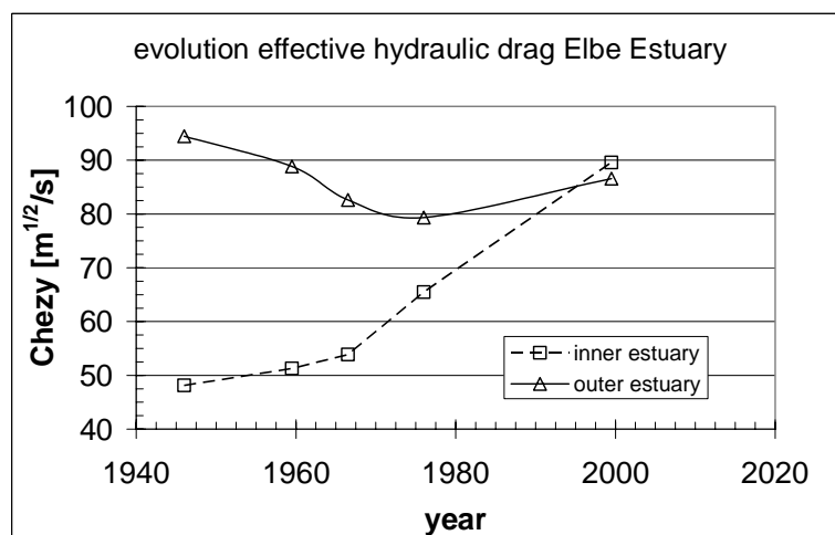
Fig. 4.30: Variation in effective hydraulic drag along the Elbe River as a result of human interventions.
