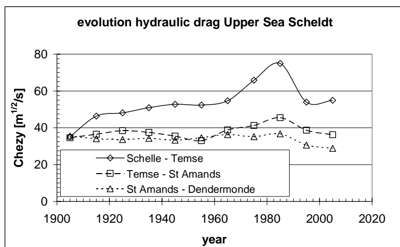
Fig. 4.54: Evolution of effective hydraulic drag (Chézy coefficient) with time,
