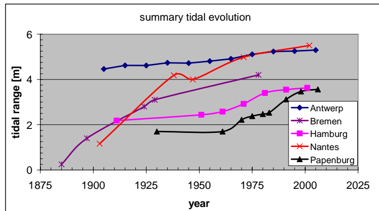
Fig. 1.1: Tidal evolution in five European ports (Antwerp along Scheldt, Belgium; Bremen along Weser, Germany; Hamburg along Elbe, Germany; Nantes along Loire, France; and Papenburg along Ems, Germany).
