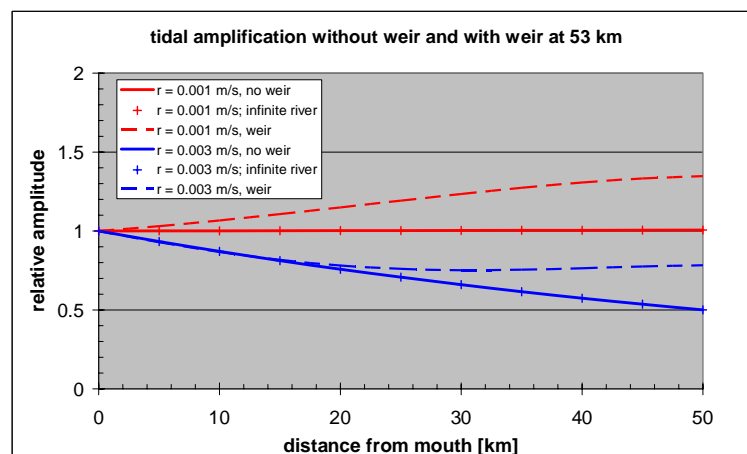
Fig. 2.4: Evolution of tidal wave in short converging estuary ( \ell = 53 km, L_b = 33 km); r = 0.00001 m/s yields C \approx 300 m^{1/2}/s ; r = 0.001 m/s yields C \approx 100 m^{1/2}/s ; r = 0.003 yields C \approx 60 m^{1/2}/s .
