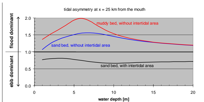
Fig. 5.3: Response of tidal asymmetry ( \gamma -parameter) as function of the presence of an intertidal area and mud in the water column, or on the River bed.
