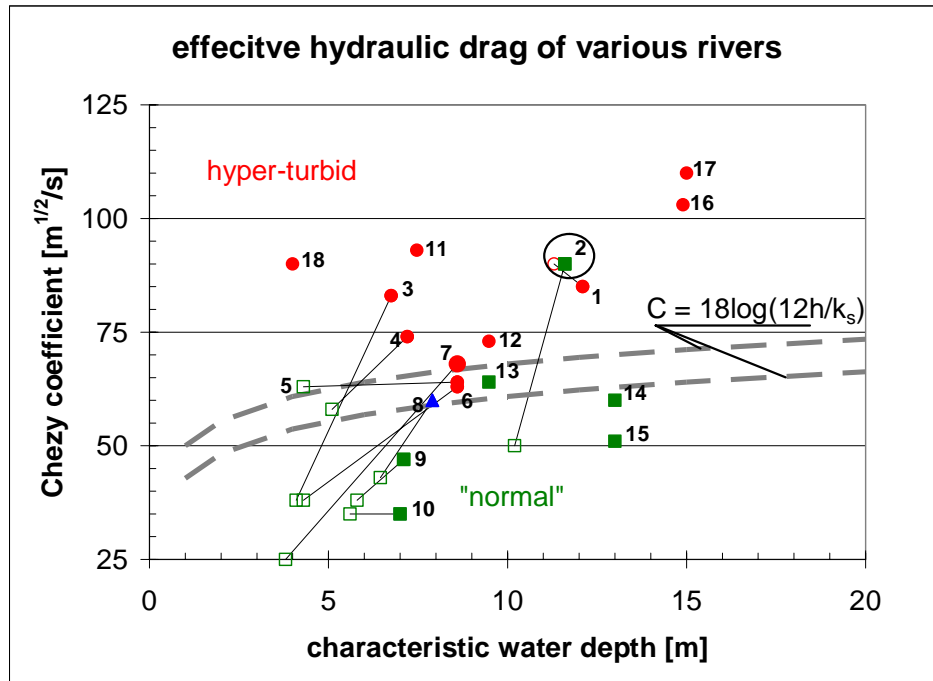
Fig. 5.8: Comparison of effective hydraulic drag in some rivers as a function of water depth. The C - h relation is based on k_s = 2 and 5 cm, arbitrary values. Red symbols depict hyper-turbid conditions, green symbols "normal conditions, and blue symbols possibly transitional systems; open symbols reflect historical data. 1: Elbe-outer; 2: Elbe-inner; 3: Ems/E-L; 4: Ems/L-P; 5: Loire/P-C; 6: Loire/C-laM; 7: Loire/LaM-N; 8: Scheldt/S-T; 9: Scheldt/T-StA; 10: Scheldt/StA-D; 11: Thames; 12: Severn-inner; 13: Severn-outer; 14: Western Scheldt; 15: Gironde-outer; 16: Gironde-inner (Villaret et al., 2011); 17: Yangtze estuary; 18: Vilaine (Vested et al., 2013). Note that data on Elbe-inner may be spurious because of tidal reflections, as discussed in Section 2. Furthermore it is presumed that the turbidity maximum in the Loire River used to be located in the outer Loire (pt 5).
