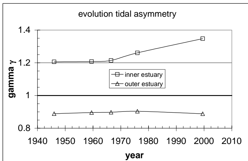
Fig. 4.34: Temporal variations in tidal asymmetry parameter \gamma in inner and outer estuary.
