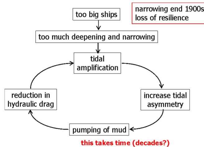
Fig. 5.4: The feed-back loop (snowball effect) for deepening of low-resilient estuaries.
