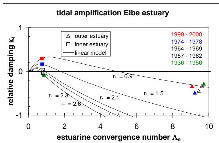
Fig. 4.29: Evolution of dimensionless tidal damping in Elbe River; the five data points and lines for the inner estuary represent the various fairway depths within the five time windows inserted in the graph (e.g. Fig. 4.25).
