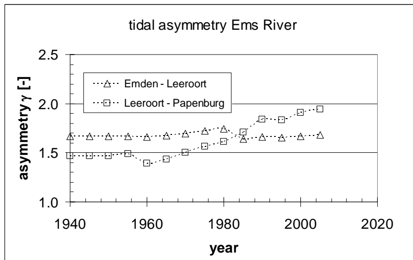
Fig. 4.11: Evolution of tidal asymmetry parameter with time.
