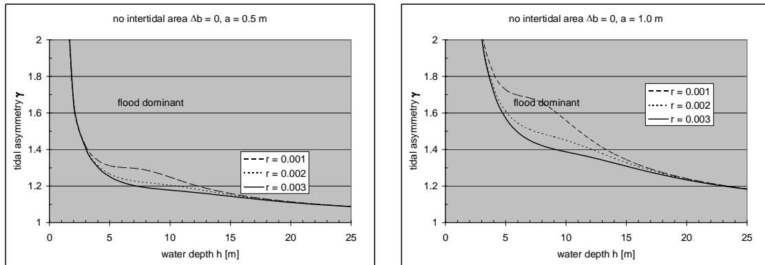
Fig. 2.10: Tidal asymmetry \gamma (= c_{HW} / c_{LW}) without intertidal area.
