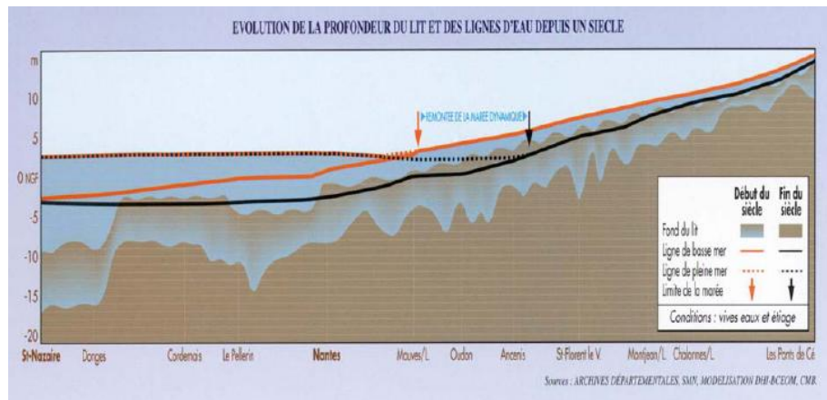
Fig. 4.14: Evolution of the river bed in the Loire River (after Sogreah, 2006).
