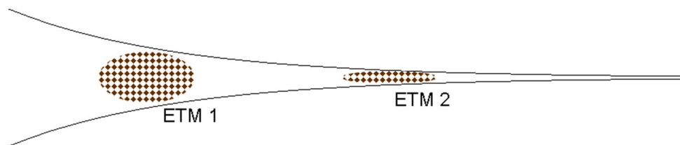
Fig. 5.1: Sketch of Estuarine Turbidity Maximum (ETM); ETM is characterized by a balance between river-induced flushing and estuarine circulation (and some tidal asymmetry), and ETM2 by a balance between the effects of river-induced flushing and tidal asymmetry.
