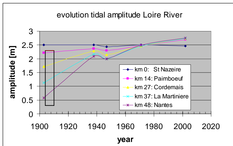
Fig. 4.17: Evolution of the tidal amplitude along the Loire River; the black box represents the period of river narrowing (e.g. Fig. 4.13).
