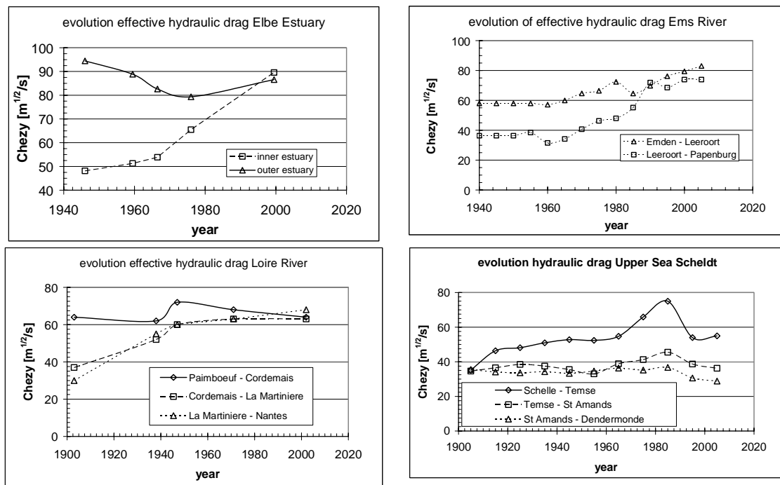
Fig. 5.7: Summary of evolution of computed Chézy coefficient with time for four European rivers.
