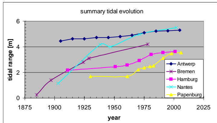
Fig. 5.5: Summary of tidal amplification in the 19th century in a number of European ports.
