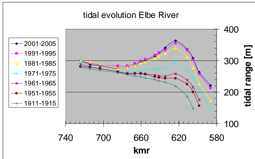
Fig. 4.23: Tidal amplification as function along Elbe River (after Weilbeer and Klöpffer, 2011)
